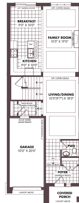
GROUND FLOOR ELEVATION A & C
