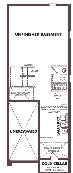
BASEMENT ELEVATION A & C
